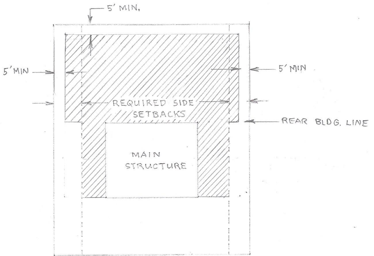
Figure A. Allowable area for small accessory structures (<150SF) on small (<1acre) lots.
