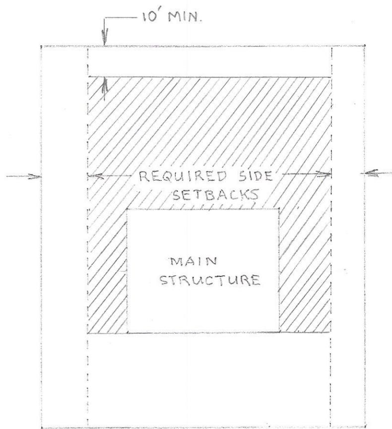
Figure C , Allowable area for all accessory structures on large ( \geq 1 acre) lots
