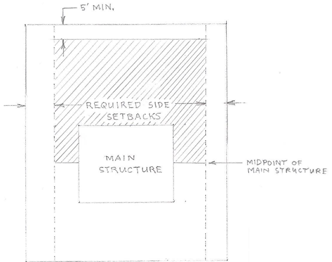
Figure A . Allowable area for small accessory structures (< 150 SF) on small (< 1 acre) lots.
