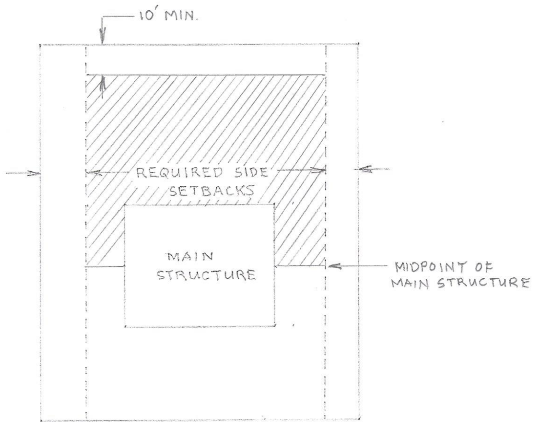
Figure C , Allowable area for all accessory structures on large ( \geq 1 acre) lots
